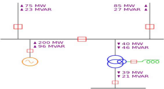
A typical one-line diagram with annotated power flows.
