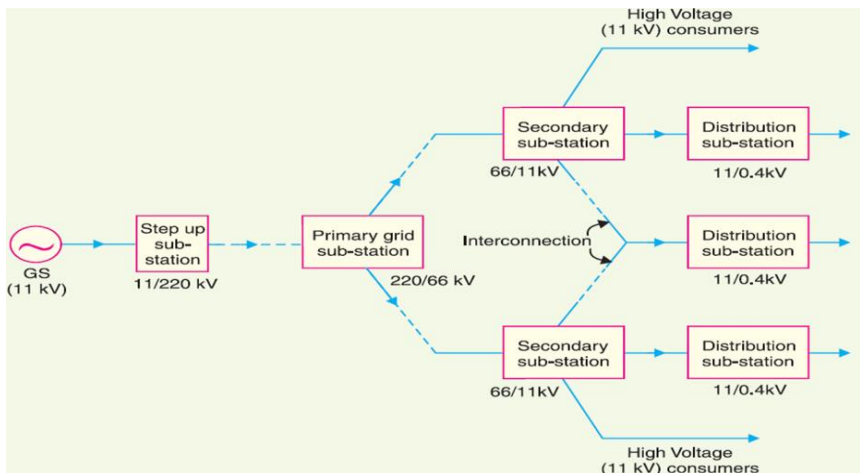
Block diagram of feed-in at a substation
