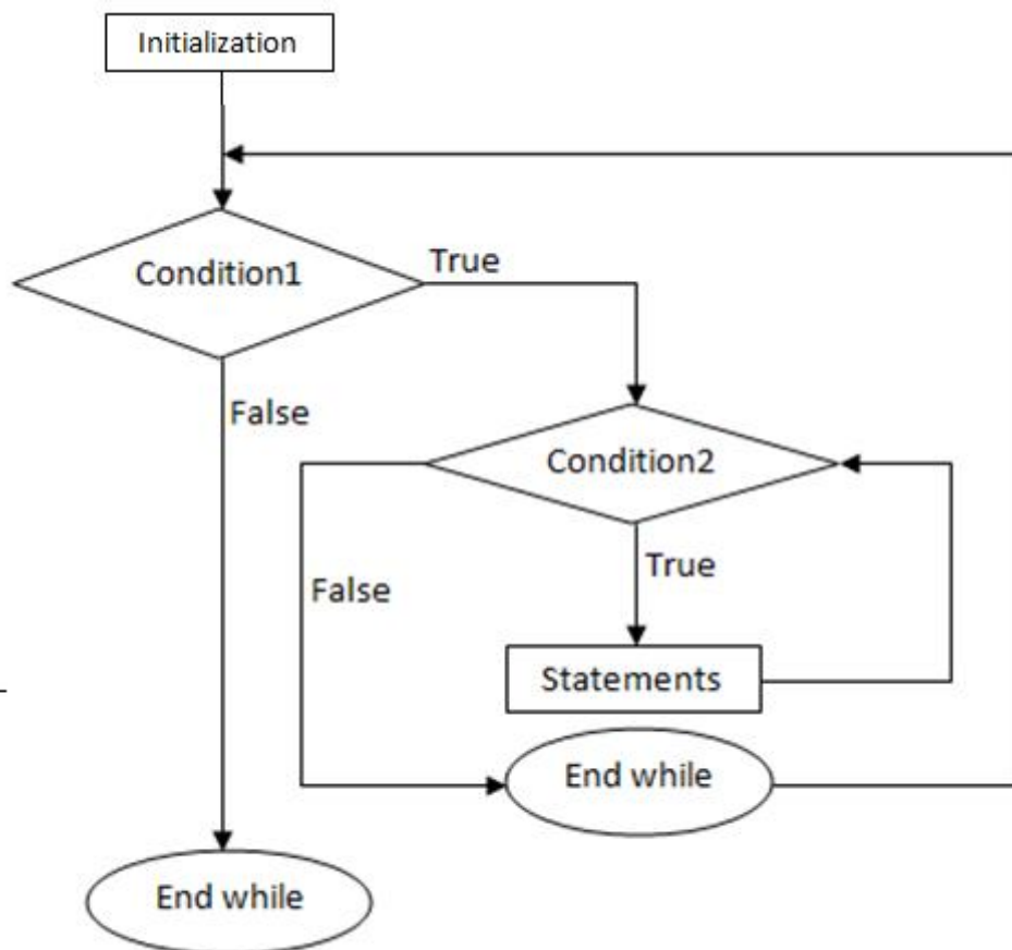
fig: Flowchart for nested while loop
