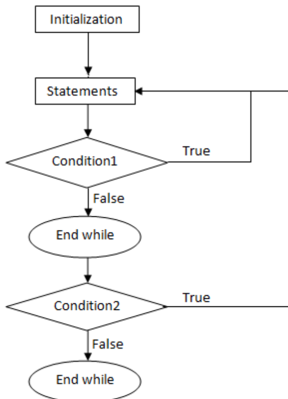
Fig: Flowchart for nested do-while loop
